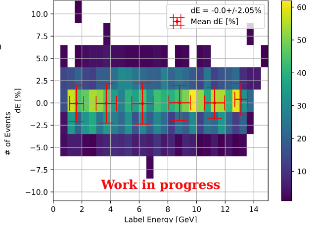
Figure 7: Difference between label and predicted visible energy in percentage, after bias correction. Overall mean and standard deviation are 0.0 \pm 2.05\% .
