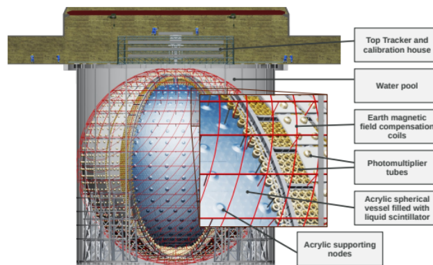
Figure 1: Schematic view of the JUNO detector.
