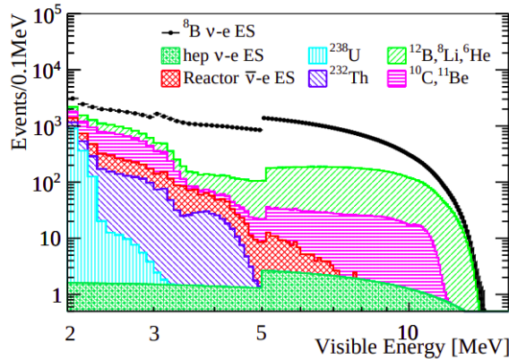
Figure 2: Expected signal and background spectra in ten years of data taking, with all selection cuts and muon veto methods applied. Figure extracted from [4].
