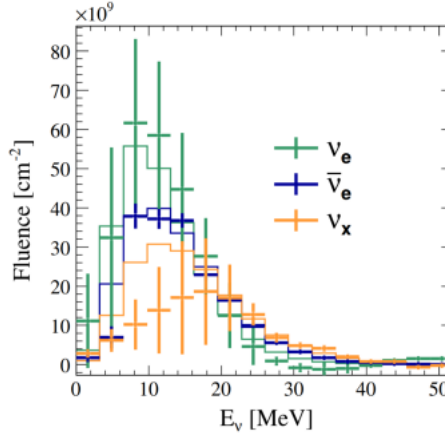
Figure 7: Reconstructed neutrino spectrum for each neutrino flavor, assuming a SN at 10 kpc. Fig. from [9].
