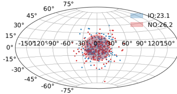
Figure 6: Skymap of the reconstructed CCSN localisation. The shaded region represents the the 68% CL area, for a CCSN with Galactic coordinates (0,0). The points represent 200 realisations of a CCSN simulated for each neutrino mass ordering hypothesis (inverted in blue, normal in pink).
