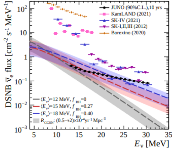
Figure 4: JUNO 90% confidence level upper limits on the DSNB fluxes for 18 equal neutrino energy bins in the range [12,30] MeV. The grey, red and blue bands with dashed lines show the DSNB flux predictions for different model parameters, with its corresponding uncertainties. JUNO sensitivity is compared to the current limits by Kamland, Borexino and SK experiments.
