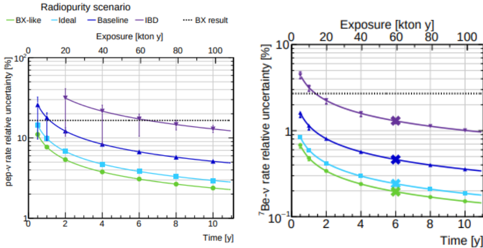
Figure 3: Relative uncertainties on the measurement of the pep (left) and ^7\text{Be} neutrino rate (right) as a function of exposure. The results for the four radiopurity scenarios are shown respectively in different colors. The best result by Borexino (17%) is indicated by the black dotted line for comparison.
