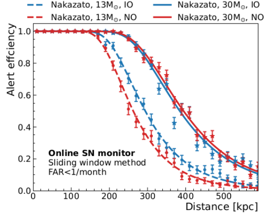
Figure 5: Alert efficiency of the online SN monitor as function of the distance to the source, using the sliding window method. Two different progenitor masses are considered, as well as the normal and inverted neutrino mass ordering scenarios.
